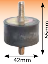
Bonnet Mounting
