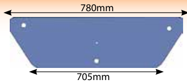
Glass 300 Bottom Rear Window
