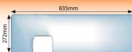
Glass IHC XL Lower Rear Window
