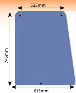
4593 Glass Ford Super Q Side Glass
