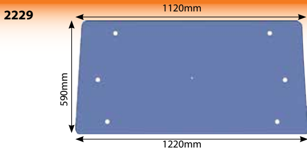
Glass 300 Rear Window Silver Cab
