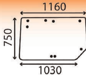
780186 Glass Rear Window Renault Ceres Series OE Ref: 6005023210
