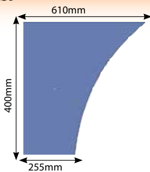
Glass 300 Short Bottom Door
