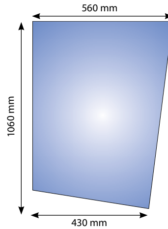
30281 Glass JCB Pro 8 Side RH
