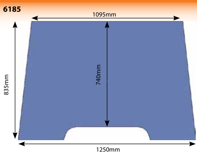
Glass 300 Windscreen - Silver Cab
