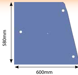
Glass 300 Side Glass - 600 x 580mm
