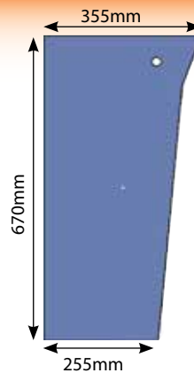
Glass 300 LH Lower Front + Holes
