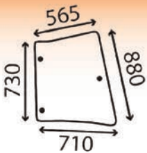
780182 Glass Rear Corner RH Renault Ares RX RZ Serie OE Ref: 7700054133
